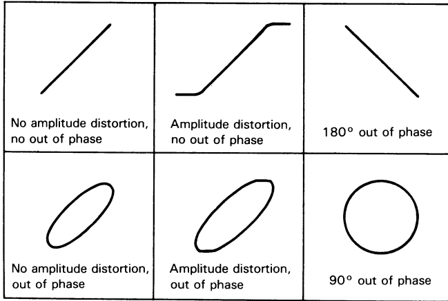
Fig. 26 Typical phase measurement oscilloscope displays
