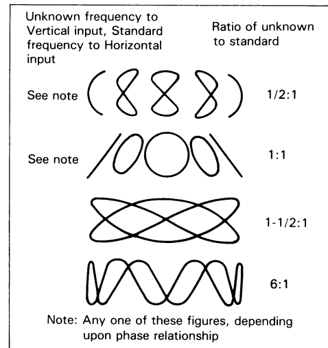
Fig. 27 Lissajous waveforms used for frequency measurement
