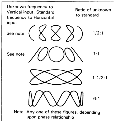
Fig. 27 Lissajous waveforms used for frequency measurement
